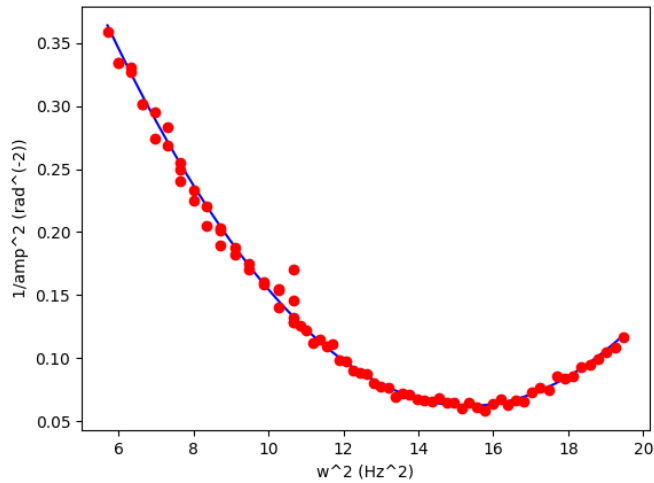
<figure 12: A^{-2} vs w^2 fitting: 5mm>
